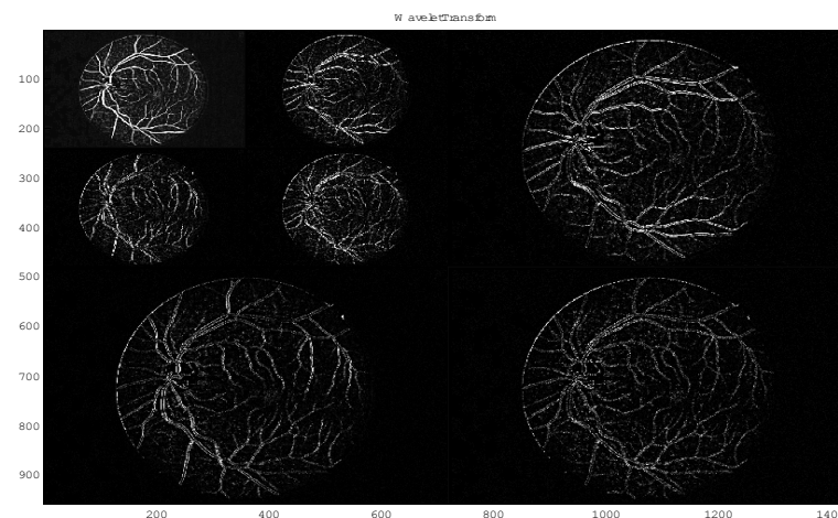
Figure 6. Wavelet decomposition.
